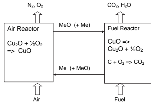
Fig. 4. Chemical-Looping with Oxygen Uncoupling (CLOU) using CuO/Cu 2 O. The fuel is carbon.
