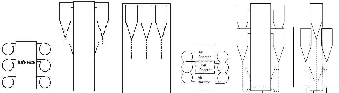
Figure 10. Left: layout of 1000 MWth FBC boiler, Right: Layout of 1000 MWth CLC boiler. From [63].
