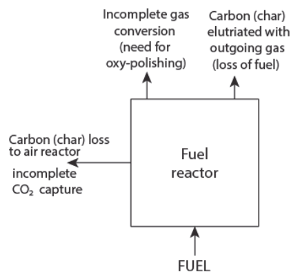
Figure 5. Inadequate performance of the fuel reactor.
