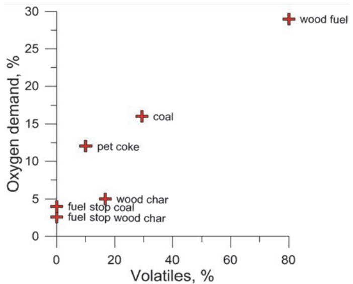
Figure 6. Oxygen demand vs volatiles in 100 kW unit
